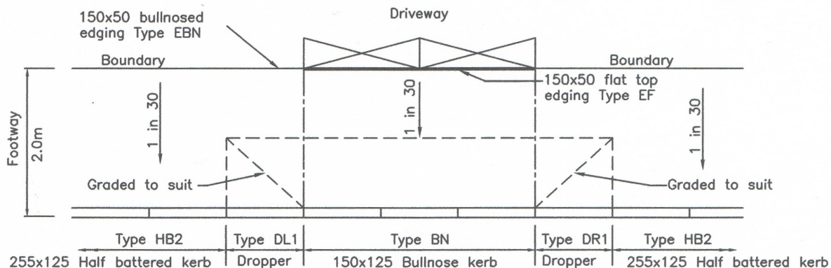
PLAN OF VEHICULAR CROSSOVER
