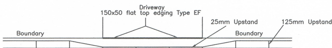
ELEVATION OF VEHICULAR CROSSOVER
